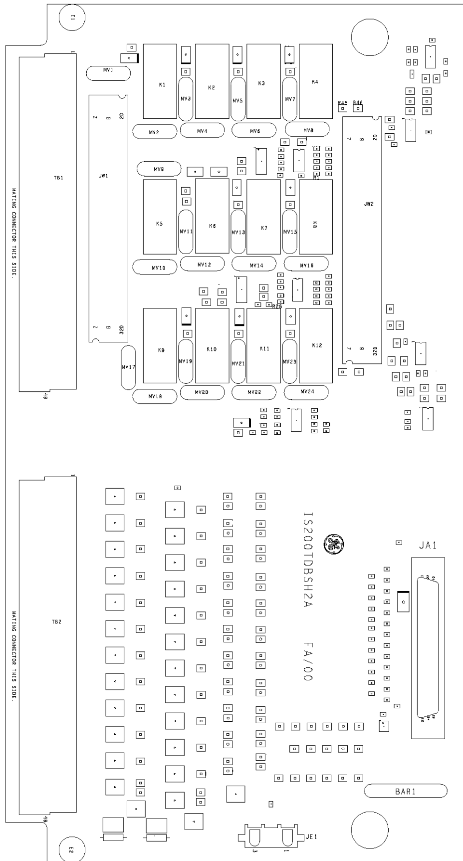
TDBS Layout
